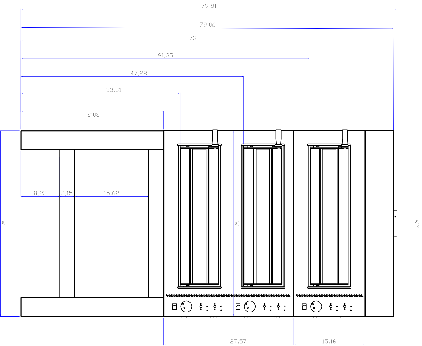
FRONT VIEW
