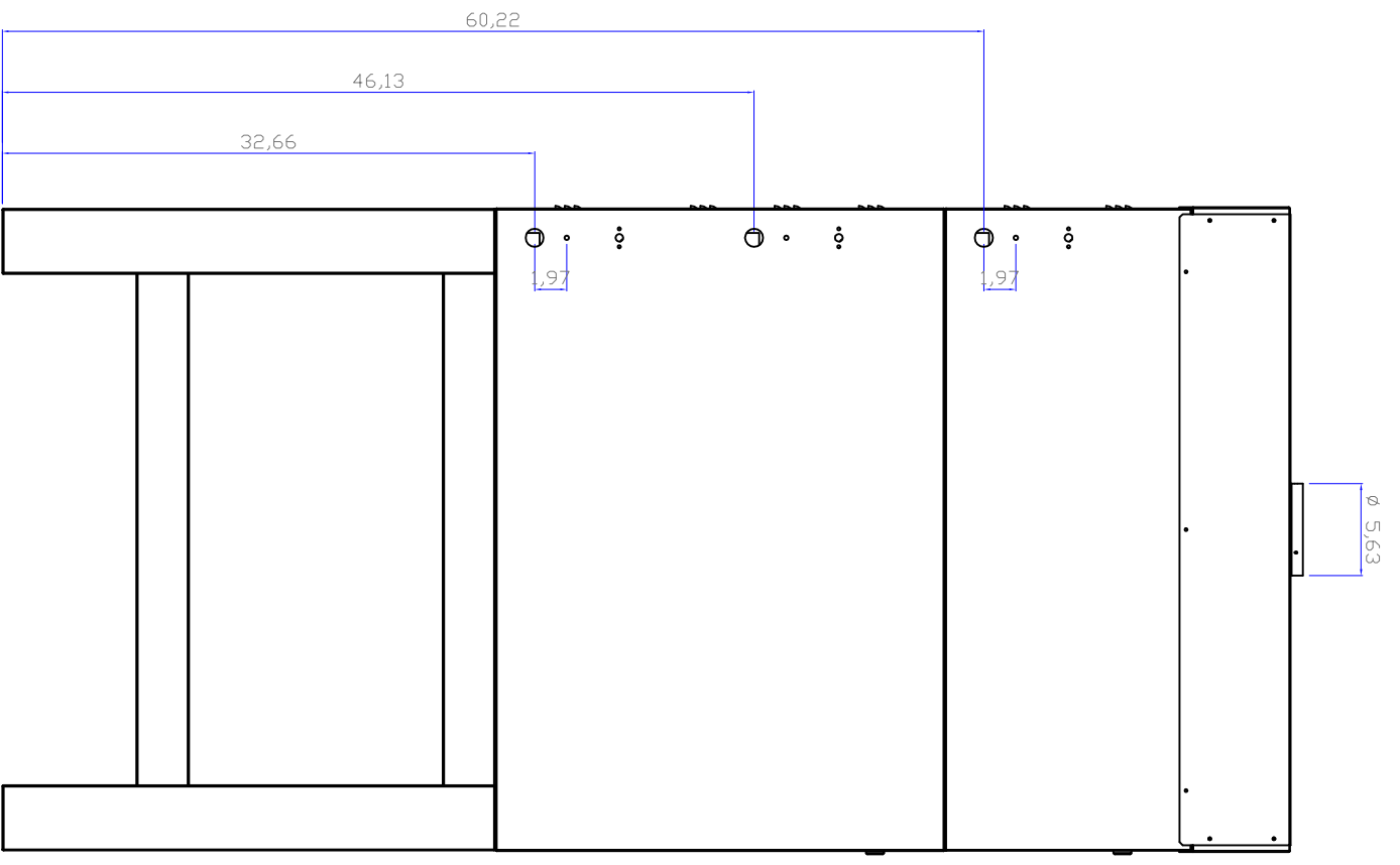
BACK VIEW
