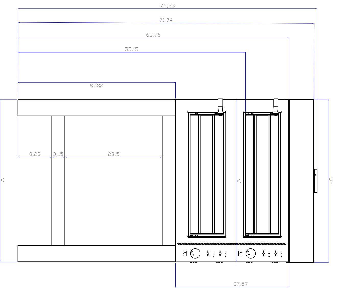
FRONT VIEW
