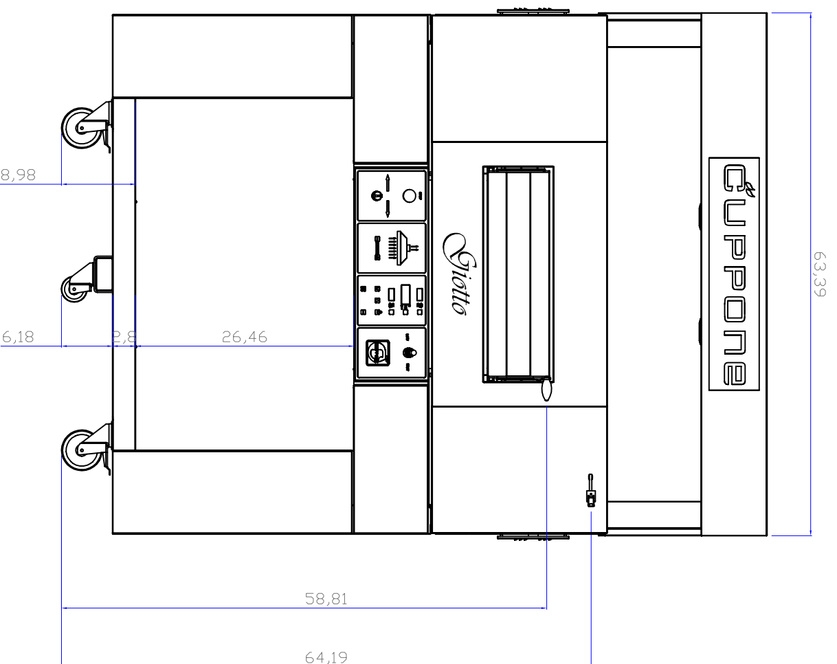
FRONT VIEW
