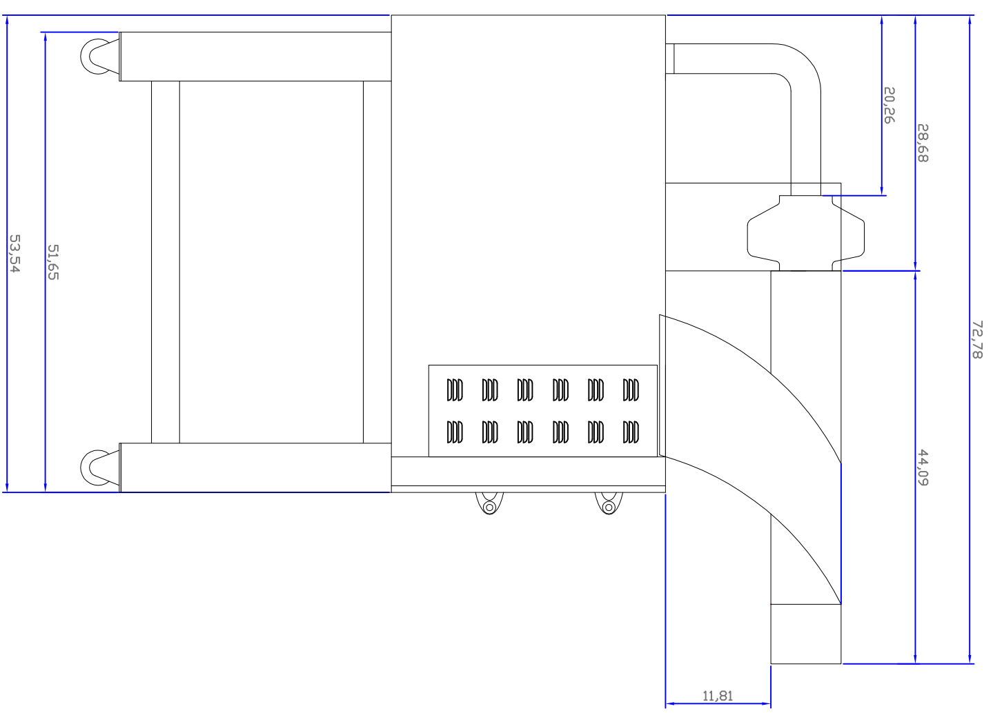
SIDE VIEW
