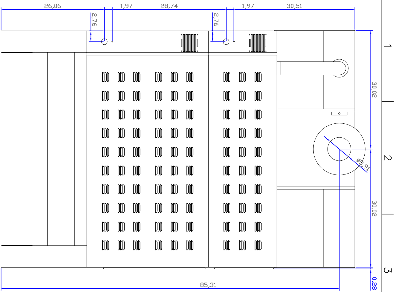
BACK VIEW
