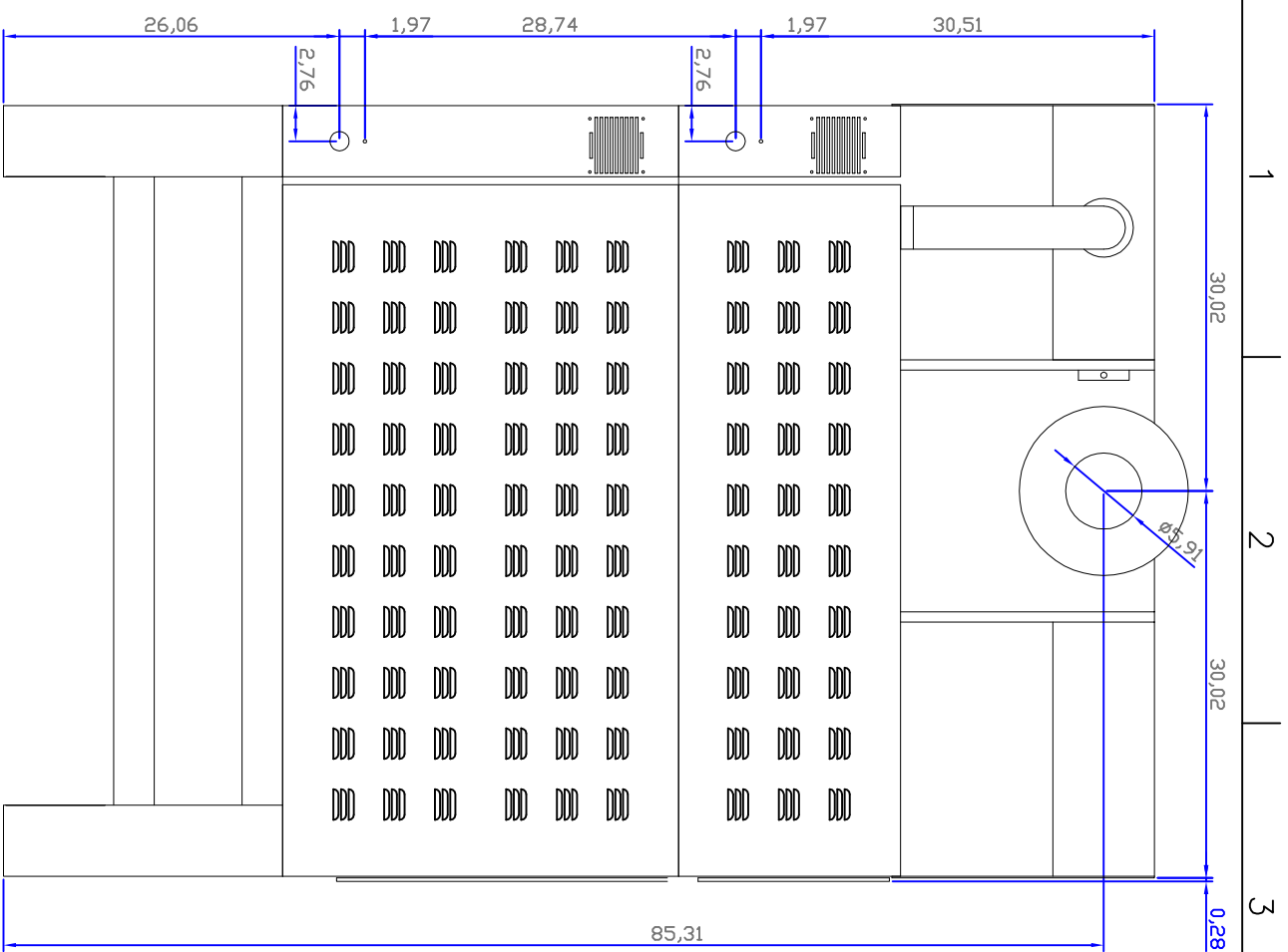
BACK VIEW
