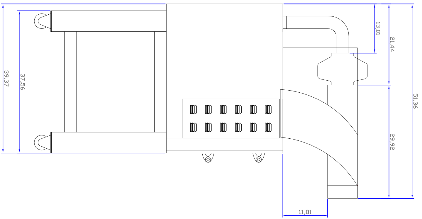
SIDE VIEW
